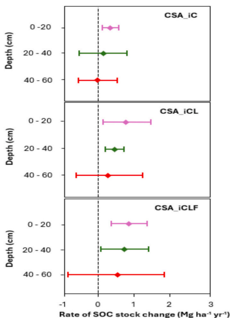
Fig. 5. Influence of depth on the rate of change of carbon stocks in CSA systems. The broken black line represents the boundary between a positive and a negative response to the response ratio. Effect sizes were considered significant if 95% Confidence intervals (CI) did not overlap zero. Definition of abbreviations: CSA represents Climate-Smart Agriculture, iC represents integrated cropping, iCL represents integrated crop-livestock, and iCLF represents integrated crop-livestock-forest.
