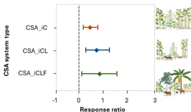
Fig. 2. Influence of CSA systems on the natural logarithm of the response ratio to rates of soil carbon change in Rondônia State, Brazil. The black broken line represents the boundary between a positive and negative response to the response ratio (RR). Effect sizes were considered significant if 95% Confidence intervals (CI) did not overlap zero. Definition of abbreviations: CSA represents Climate-Smart Agriculture, iC represents integrated cropping, iCL represents integrated crop-livestock, and iCLF represents integrated crop-livestock-forest.
