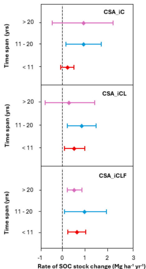
Fig. 3. Effects of time on SOC stock rate change in the CSA systems. The broken black line represents the boundary between a positive and negative response to the response ratio (RR). Effect sizes were considered significant if 95% Confidence intervals (CI) did not overlap zero. Definition of abbreviations: CSA represents Climate-Smart Agriculture, iC represents integrated cropping, iCL represents integrated crop-livestock, and iCLF represents integrated crop-livestock-forest.
