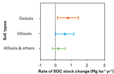
Fig. 8. Effect of soil types on SOC stock rate change in the CSA systems. The broken black line represents the boundary between a positive and negative response to the response ratio. Effect sizes were considered significant if 95% Confidence intervals (CI) did not overlap zero. Not all the study locations reported the main soil types ( n = 44 ). Oxisols, that is Ferralossols in the American Taxonomy, and Latossolos or Latosols in the Brazilian Taxonomy. Ultisols or Acrisols in the American taxonomy, and Argissolos in the Brazilian taxonomy.
