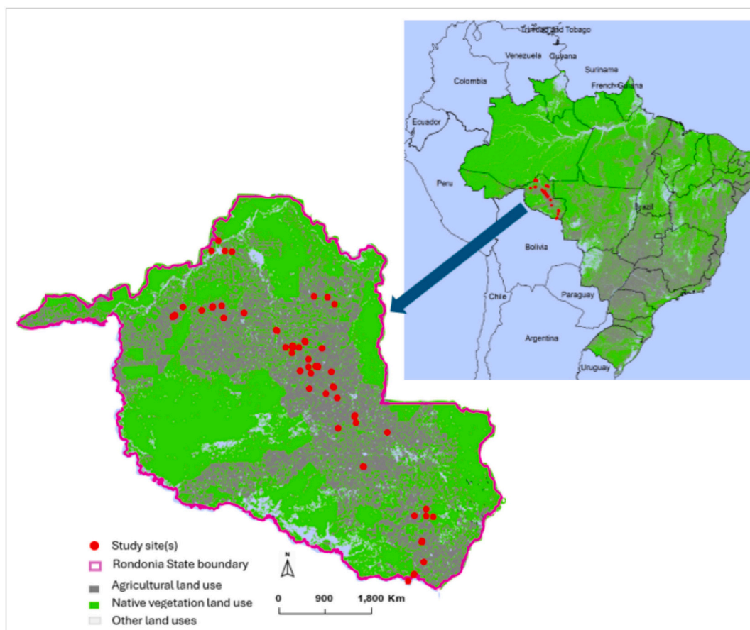
Fig. 1. Study observation data points on the SOC stocks in CSA areas in Rondônia State, Brazil. Rondônia State (lower left map), Brazil, in South America (upper right map).
