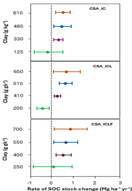
Fig. 6. Influence of clay (soil texture) on the rate of change of carbon stocks in CSA systems. The broken black line represents the boundary between a positive and negative response to the response ratio. Effect sizes were considered significant if 95% Confidence intervals (CI) did not overlap zero. Definition of abbreviations: CSA represents Climate-Smart Agriculture, iC represents integrated cropping, iCL represents integrated crop-livestock, and iCLF represents integrated crop-livestock-forest.
