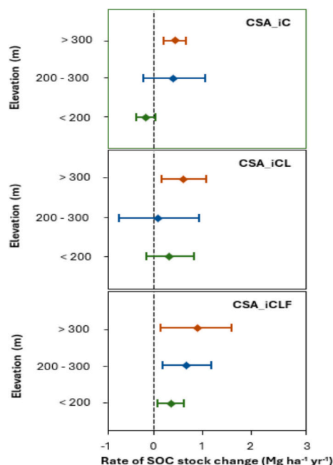
Fig. 7. Influence of elevation on the rate of change of carbon stocks in CSA systems. The broken black line represents the boundary between a positive and negative response to the response ratio. Effect sizes were considered significant if 95% Confidence intervals (CI) did not overlap zero. Definitions of abbreviations: CSA represents Climate-Smart Agriculture, iC represents integrated cropping, iCL represents integrated crop-livestock, and iCLF represents integrated crop-livestock-forest.
