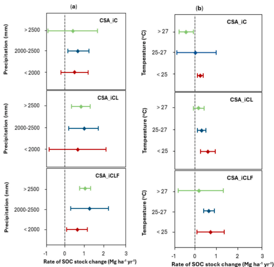
Fig. 4. Influence of climate on the rate of change of carbon stocks in CSA systems. Precipitation (Fig. 4a), and temperature (Fig. 4b). The broken black line represents the boundary between a positive and negative response to the response ratio. Effect sizes were considered significant if 95% Confidence interval (CI) did not overlap zero. Definition of abbreviations: CSA represents Climate-Smart Agriculture, iC represents integrated cropping, iCL represents integrated crop-livestock, and iCLF represents integrated crop-livestock-forest.
