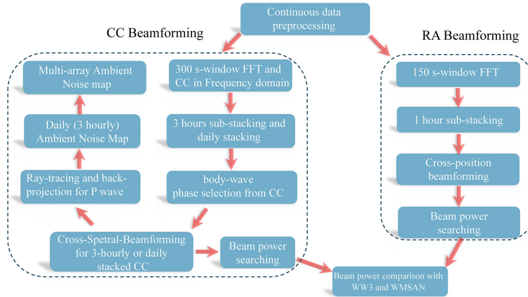
Figure 2. Workflow for retrieval of secondary microseisms from ambient noise CC beamforming and RA beamforming. CC beamforming is applied on three networks to jointly map the location of secondary microseisms and relative amplitude extraction for the geophones from ANTICS, whereas the RA beamforming is applied for the ANTICS broad-band stations to extract the absolute amplitude of secondary microseisms in the northern Atlantic.
