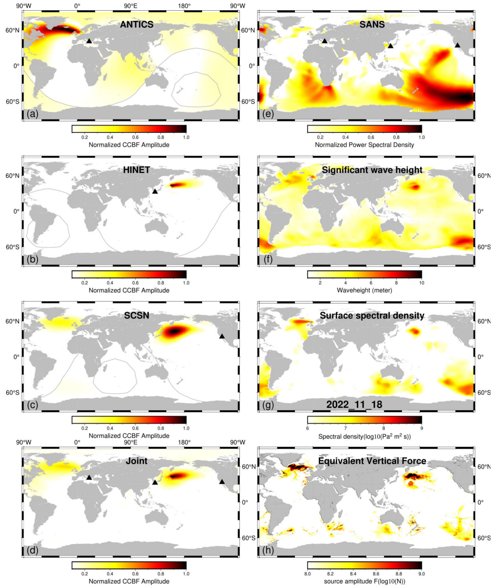
Figure 4. (a–c) Cross-correlation beam power and backprojection for three individual networks; grey curves in (a)–(c) denote epicentral distances of 90^\circ and 120^\circ . (d) Joint backprojection constraints from the three networks. (e) Seismic Ambient Noise Source (SANS) maps from full waveform inversion (J. Igel et al. 2021). (f) daily averaged wave height map on 2022 November 18 and (g) daily averaged surface spectral density at 5–10 s, as extracted from WW3 model. (h) Equivalent vertical force on the ocean floor considering the source site effects and assuming body wave propagation, reconstructed using WMSAN from L. Tomasetto et al. (2025).
