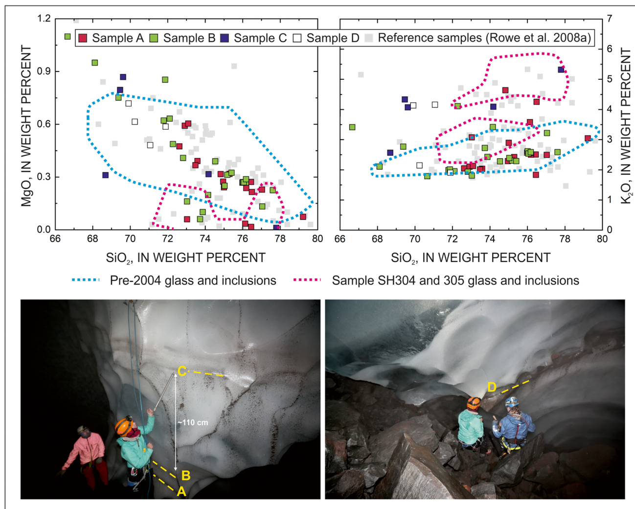
Fig. 10 Chemical variation diagrams of MgO and K 2 O versus SiO 2 contents in clean groundmass glass. Colored square symbols in the plots illustrate the different tephra layers sampled in 2021. Reference fields comprise glass and melt inclusion compositions for dome samples SH304 and SH305 from 2004/2005 explosions (dashed magenta line), as well as pre-2004 tephra and dome glass compositions (dashed blue line) (cf. Rowe et al. 2008a). Although many analyzed grains from samples A and B have compositions similar to pre-2004 tephra, a subset of grains in samples A and B (and one grain in sample C) has the distinctly lower MgO and higher K 2 O groundmass
