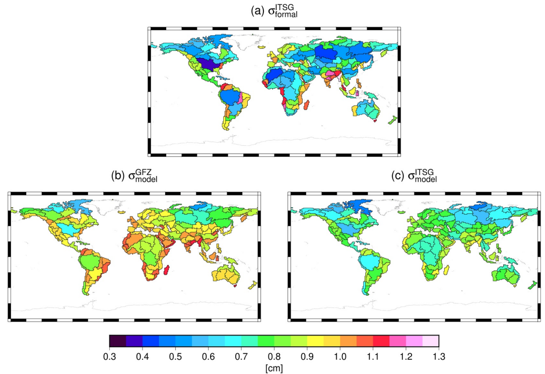
Figure 2. Long-term mean standard deviations of GRACE-based TWS for 156 basins derived from the rigorous error propagation of the ITSG-Grace2018 variance-covariance matrix of the Stokes coefficients ( \sigma_{\text{formal}}^{\text{ITSG}} ) as well as our spatial covariance model applied to ITSG-Grace2018 ( \sigma_{\text{model}}^{\text{ITSG}} ) and GFZ RL06 ( \sigma_{\text{model}}^{\text{GFZ}} ).
