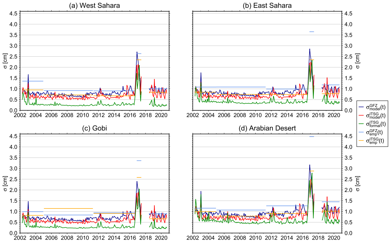
Figure 7. Time series of formal, modeled, and empirical standard deviations for four different regions in (a) West Sahara, (b) East Sahara, (c) Gobi and (d) Arabia.
