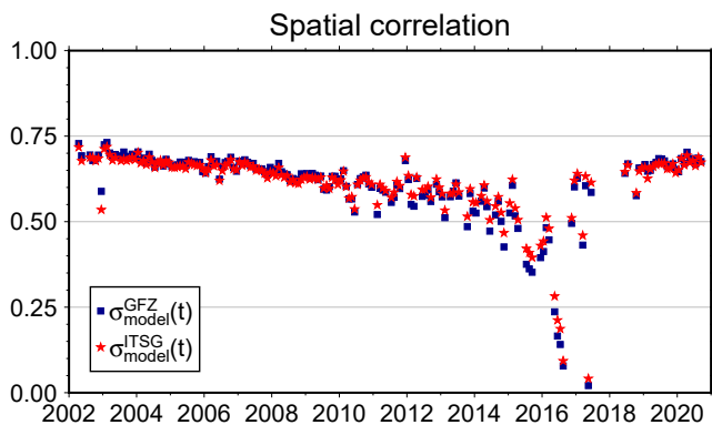
Figure 4. Spatial correlations between the maps of uncertainties for 156 discharge basins obtained from the rigorous error propagation of the ITSG-Grace2018 variance-covariance matrix of the Stokes coefficients ( \sigma_{\text{formal}}^{\text{ITSG}}(t) ) and our spatial covariance model applied to ITSG-Grace2018 ( \sigma_{\text{model}}^{\text{ITSG}}(t) ) as well as to GFZ RL06 ( \sigma_{\text{model}}^{\text{GFZ}}(t) ) for each monthly solution of the GRACE/GRACE-FO data record.
