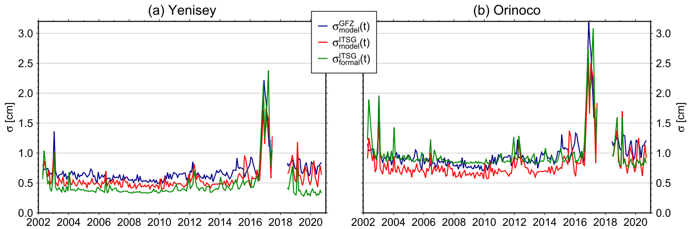
Figure 1. Monthly-mean basin standard deviations derived from the rigorous error propagation of the ITSG-Grace2018 variance-covariance matrix of the Stokes coefficients ( \sigma_{formal}^{ITSG}(t) ) as well as our spatial covariance model applied to ITSG-Grace2018 ( \sigma_{model}^{ITSG}(t) ) and GFZ RL06 ( \sigma_{model}^{GFZ}(t) ) for (a) the Yenisey and (b) the Orinoco basin.
