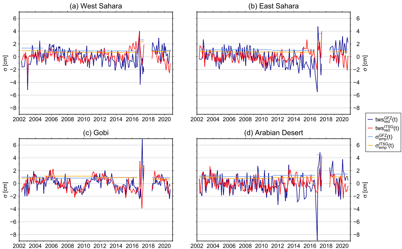
Figure 6. Residual TWS signal (i.e., trend and (semi-)annual signals removed) and resulting mean empirical standard deviations for five mission phases for four different regions in (a) West Sahara, (b) East Sahara, (c) Gobi and (d) Arabia.
