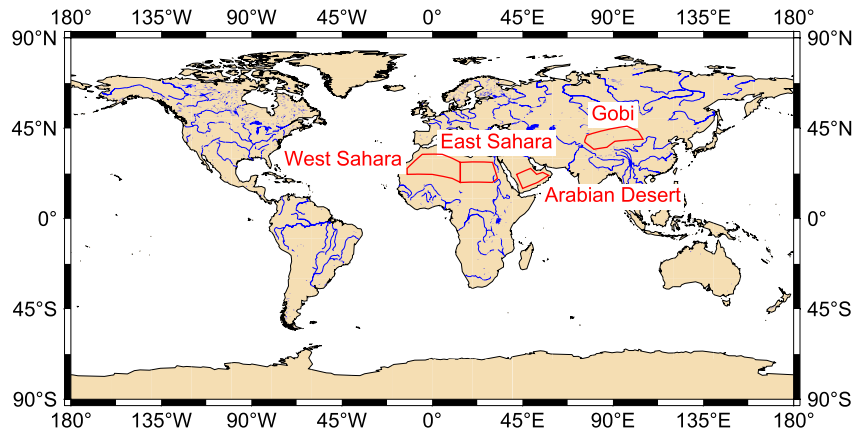
Figure 5. Polygons of the four desert regions used for the assessment of modeled uncertainties against empirical estimates.
