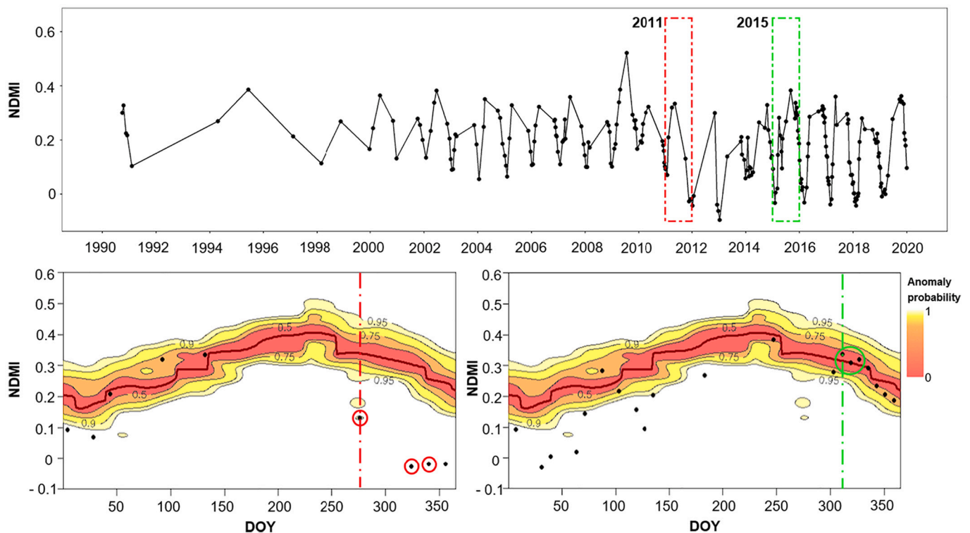
Fig. 1. The AVOCADO method for multiple disturbance and regrowth detection. A - Example of an NDMI time series for a Landsat pixel of interest (POI) in Genteguela (Ivory Coast) to be assessed. The red box delineates the data points in 2011 where the algorithm detected a disturbance with a high likelihood (outside the 95% of the reference frequency distribution or RDF \geq 0.95 ), shown in panel B, while the green box delineates the data points in 2015 where a regrowth was detected, shown in panel C). Please note that NDMI anomaly values at RDF \geq 0.95 , thus the remaining 0.05 of the RFD, are extremely high or low values. B - The reference curve of (undisturbed) forest in Genteguela representing the annual phenology and its frequency distribution (yellow colors showing which NDMI values have a high likelihood of being an anomaly) for each DOY (Day of Year) with the data points for the POI of 2011. The red circles show the consecutive data points (in this study a minimum of three points) outside the 95% of the NDMI frequency distribution ( RDF \geq 0.95 ), flagging a disturbance. C - The same reference curve as in panel B, with the data points for the POI of 2015. The green circle shows the consecutive data points (in this study a minimum of three points) which are on top or above the (dark red) reference line flagging a forest regrowth. See appendix A for the reference curves for the other sites. (For interpretation of the references to colour in this figure legend, the reader is referred to the web version of this article.)
